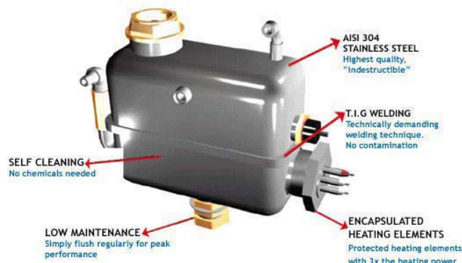
Daimer®'s Revolutionary Stainless Steel Boiler
